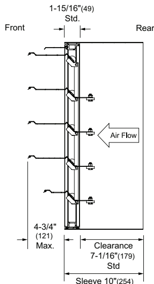
Vertical Mount with Sleeve (discharge)
