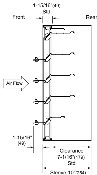
Vertical Mount with Sleeve (intake)
