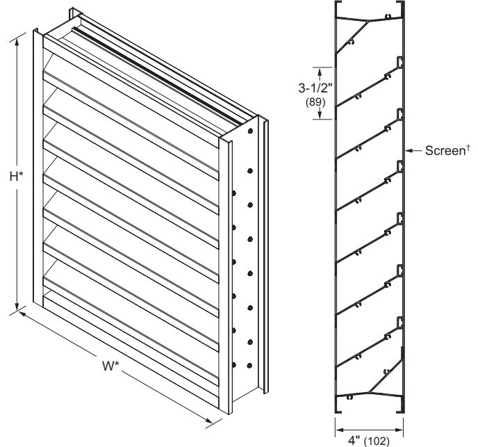
Model EFK-430 (standard)
