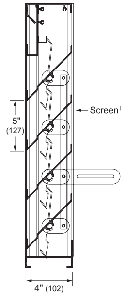
Vertical Section
