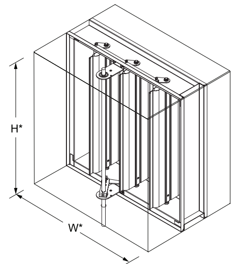
Model FSD-152V (standard)
