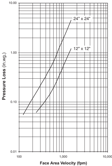
Figure 5.2 — Ducted Inlet
