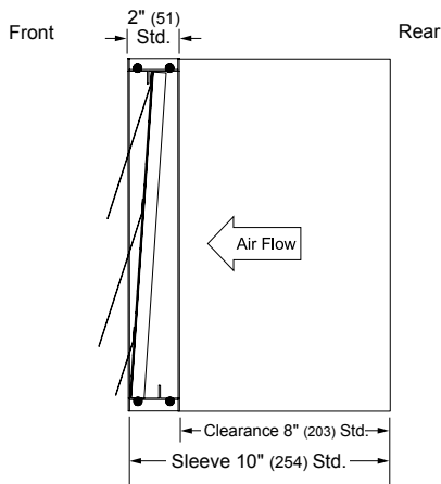
Vertical Mount with Sleeve Exhaust.
