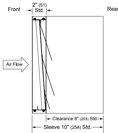
Vertical Mount with Sleeve Intake.
