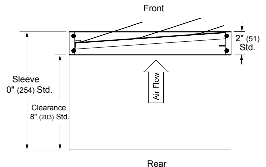
Horizontal Mount Up-flow only.
