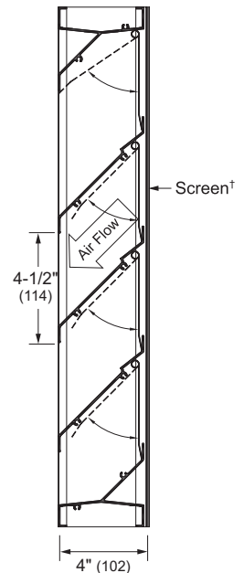
Vertical Section
