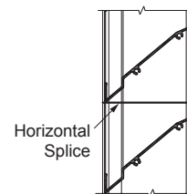
Horizontal Mullion (standard)
