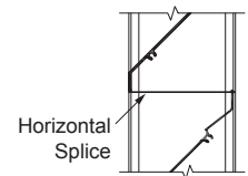
Horizontal Mullion (standard)
