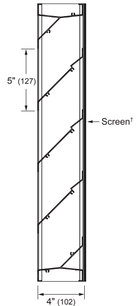
Vertical Section
