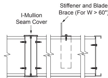
Visible Vertical Mullion (standard)
