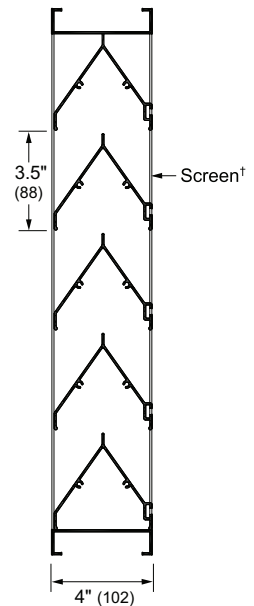
Vertical Section
