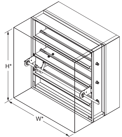
Model FSD-142 (standard)
