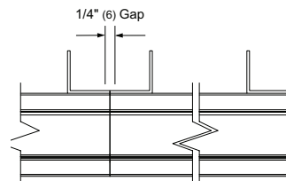
Vertical Mullion (standard)
