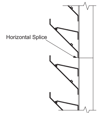
Horizontal Mullion (standard)
