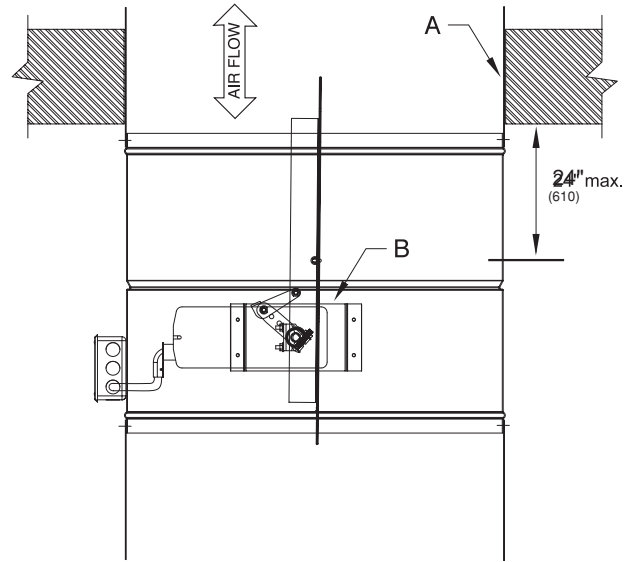
Horizontal Mount
