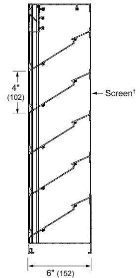
Vertical Section
