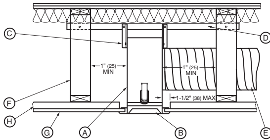
END VIEW - Duct to Grille Connection
