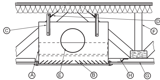
FACE VIEW
